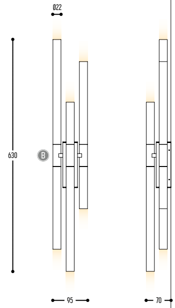
EQUALIZER Wall 3502-BB(B)-906H-K
