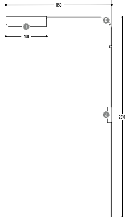
BENDIT WALL 3455-BB(B)-H-II(I)-JJ(J)-K
