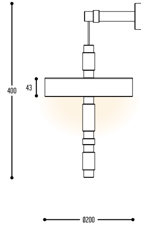
TOTM Wall 3265-COL-14H-K
